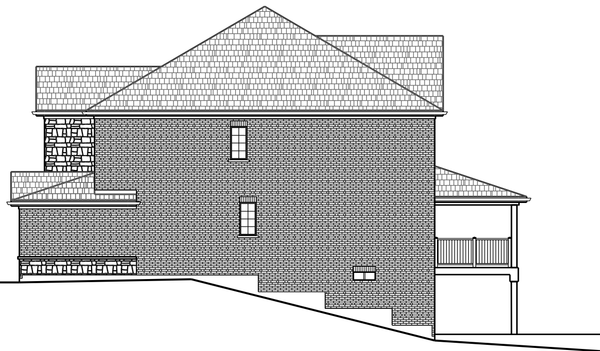
Right Side ( North ) Elevation
